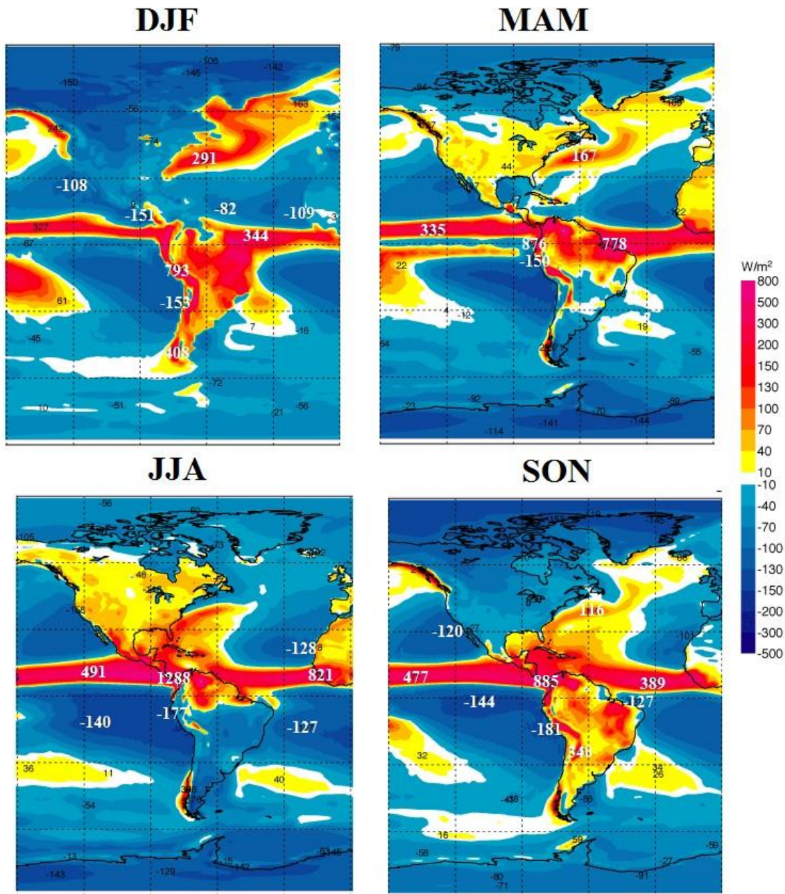
Figure S3. Figure S3. Column-integrated heating. ERA-40 Atlas
