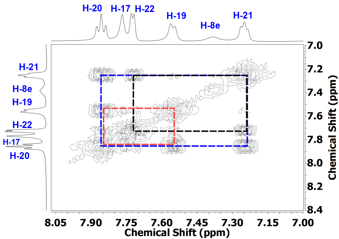
Figura 7S. 2D-NMR COSY ( \text{CD}_3\text{CN}-d_3 , 400 MHz) of grid complex [\text{Zn}_4\text{L}_4] \cdot 8(\text{BF}_4) . Aromatic region onset.
