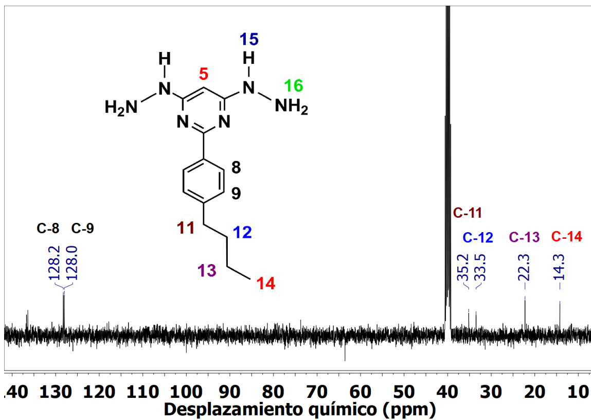
Figure S1. 13 C-NMR (DMSO- d 6 , 101 MHz) spectrum of 2-(4-butylphenyl)-4,6-dihydrazinylpyrimidine.
