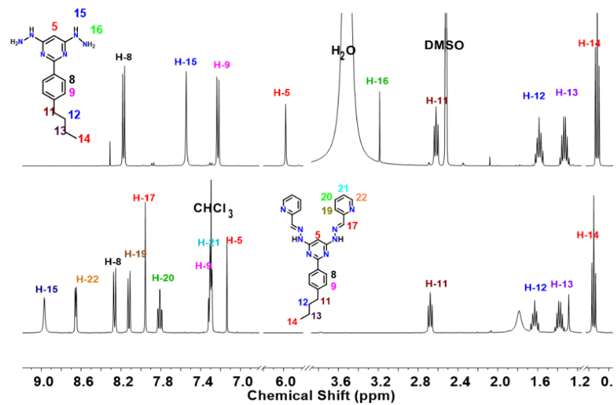
Figure S1. ^1\text{H} NMR of compounds 2 (400MHz, \text{DMSO}-d_6 ) and 3 (400MHz, \text{CDCl}_3 ).
