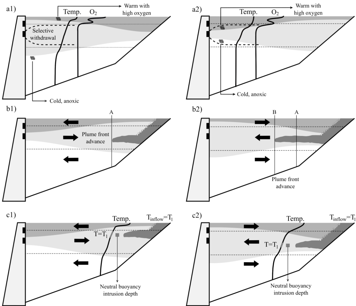
Figure S2. Schematic view of hypothetical mechanisms that could link basin-scale internal waves and water quality in Porce II reservoir.
