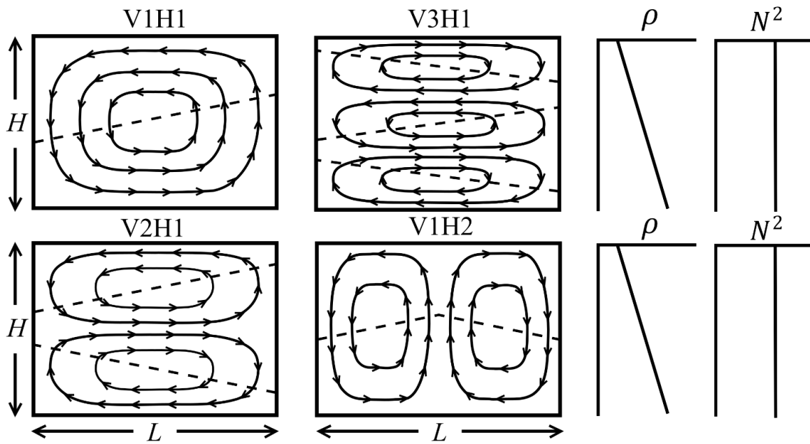
Figure S1. Schematic view of the structure of various internal wave modes for a rectangular basin of depth and length with uniform stratification.
