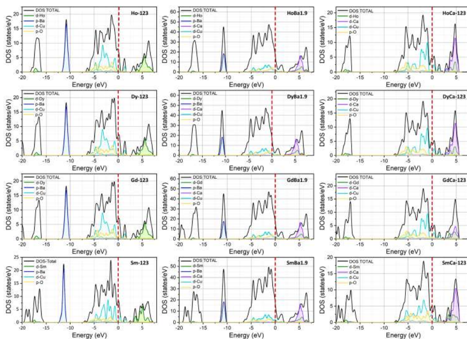
Figure 3. Density of states calculated for REBa_2Cu_3O_7 (RE-123), REBa_{1.9}Ca_{0.1}Cu_3O_7 (REBa1.9), and RECa_2Cu_3O_7 (RECa-123) superconductor systems with RE = Ho, Dy, Gd, and Sm
