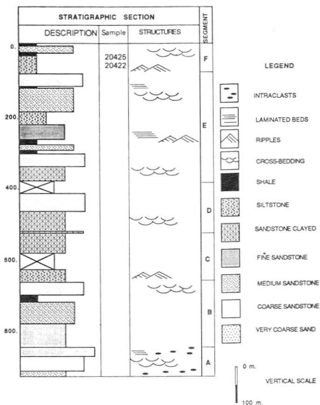
Figura 3. General Stratigraphic column of the Murca Formation. (Moreno, 1989).
