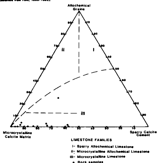
Figure 8. Ternary plot of Rosablanca Formations. The triangular Grains, Matrix and Cement plot shows the mean Limestone classification (modified from Folk, 1959, 1962).
