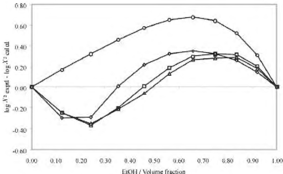
Figure 2. Logarithmic differences of drugs solubilities [experimental value minus calculated value according to Yalkowsky-Roseman model (equation 1)] for IMC (□), naproxen (◇, taken from Vargas, E. et al. (2008)), and ketoprofen (△, taken from Gantiva, M. et al. (2009)) and logarithmic difference of calculated solubilities [value according to Jouyban-Acree model (equation 5) minus value according to Yalkowsky-Roseman model (equation 1)] (○), as a function of the EtOH proportion in EtOH + water mixtures at 298.15 K.
