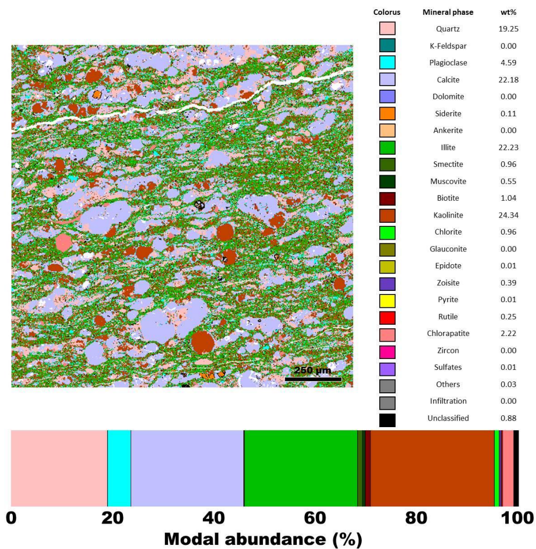
Figure 6S. Left, QEMSCAN mineral map (0.7 \mu\text{m} pixel spacing) of the selected area in Figure 2b. Right, legend indicating the recognized mineral phases. Below, the calculated modal abundances in wt%.
