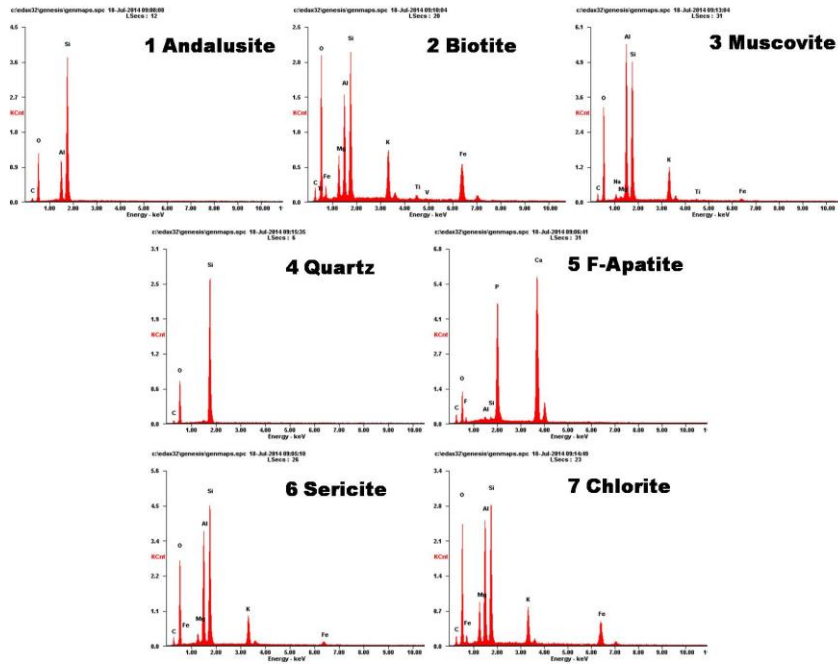
Figure 4S. Backscattered electron (BSE) image and EDS spectra at the marked stars on the image of a relictic andalusite porphyroblast (andalusite-cordierite facies). The appearance of C element is attributed to the carbon coating on the sample before SEM analysis.
