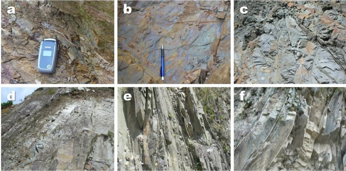
Figure 1S. Field photographs of the lithostratigraphic features observed in the western (a)-(c), central (c)-(e) and eastern (f) stripes of the Silgará Formation at the NSM.
