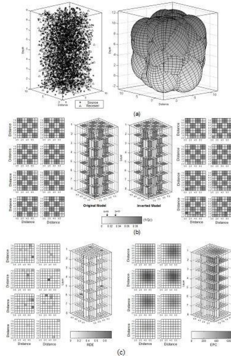
Figure 3S. Synthetic test of a pattern of contrasting attenuation in 3D. (a) Foci pairs distribution and sampling ellipsoids; (b) Original model of areas of attenuation (left), and solved model by inversion (right); (c) Distribution of the diagonal elements of the resolution matrix (left) and the number of ellipsoids crossing each block (right).
