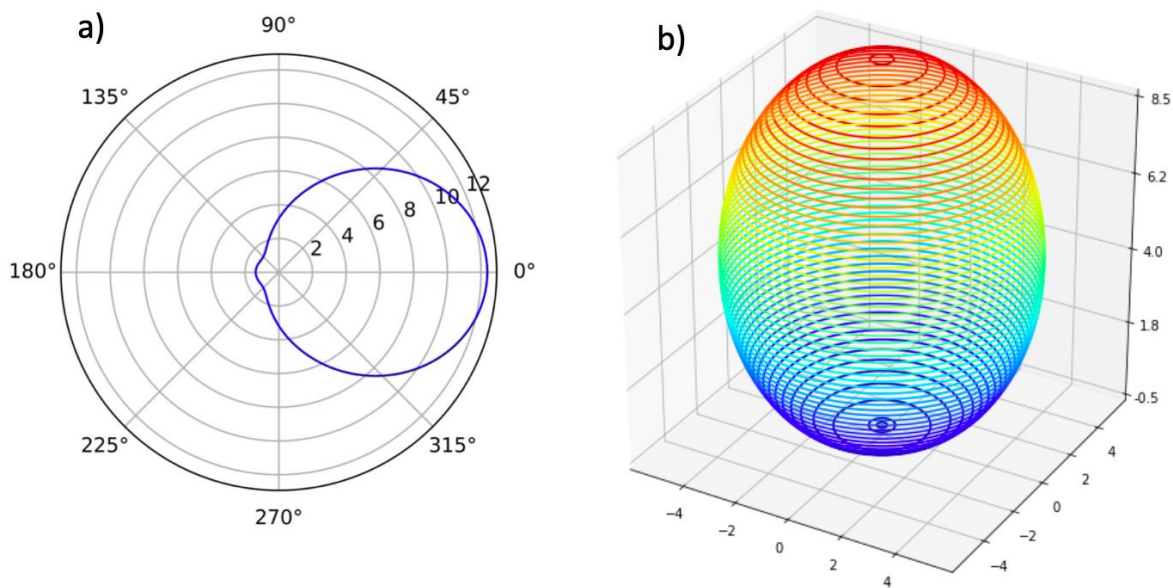
Figure 6S. Parallel and perpendicular irradiance of a Silicon nanoparticle with a radius of 80 nm in quartz, with a wavelength of 645 nm, n=3.850 , and k=0.015 . a) in polar coordinates b) in spherical coordinates.
