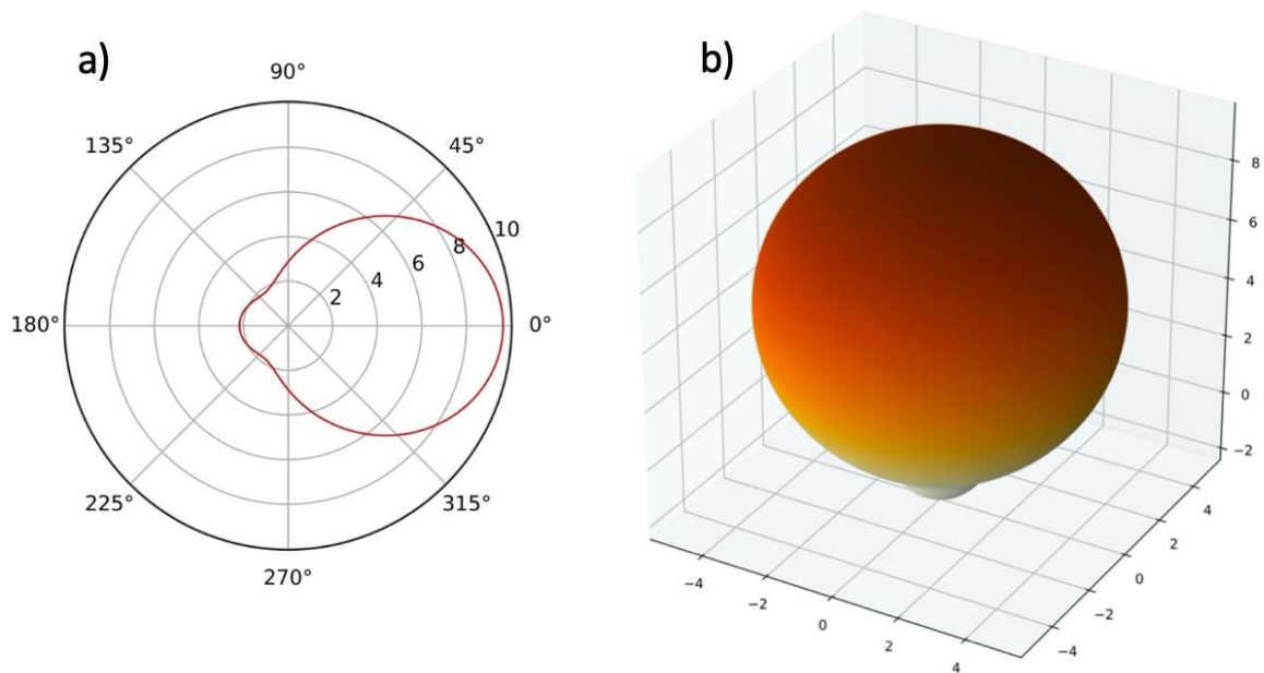
Figure 5S. Figure 5S. Parallel and perpendicular irradiance of a suspended in methanol silicon nanoparticle with a radius of 80 nm, at 645 nm wavelength, n=3.850 , and k=0.015 . a) in polar coordinates b) in spherical coordinates.
