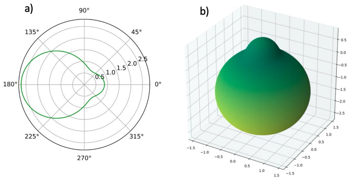
Figura 2S. Parallel and perpendicular irradiance of a Silicon nanoparticle with radius 80nm, with a wavelength of 585nm, n=3.971 y k=0.022 , a) in polar coordinates b) in spherical coordinates.
