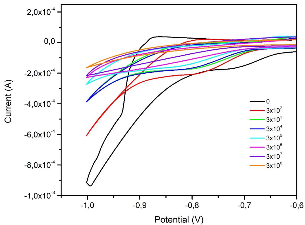
Figure 1S. Cyclic voltammetry response of SPGE-cys-GGP different concentrations of S. aureus in 1 mM \text{H}_2\text{O}_2 , scan rate 50 \text{ mV s}^{-1}
